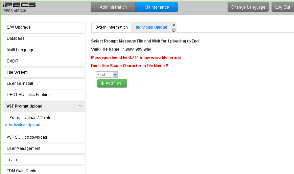
Figure 4.5.8.2-1 Individual Upload
