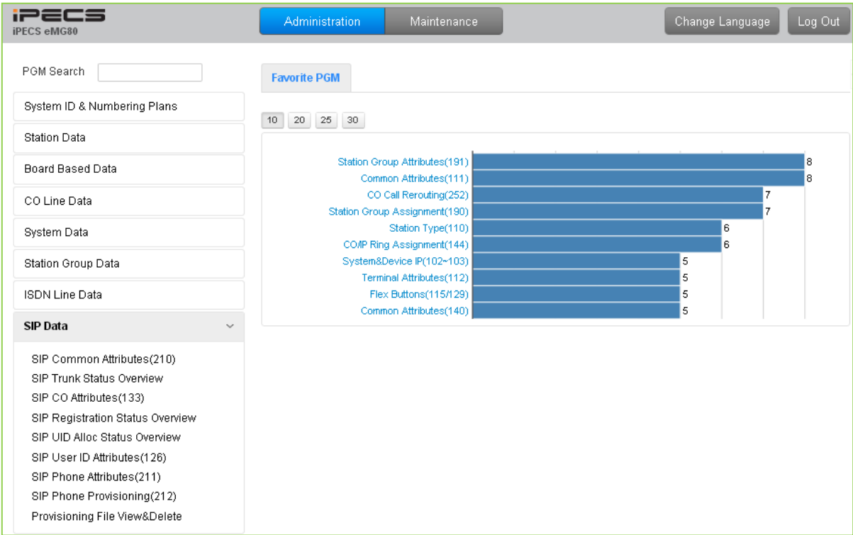
Figure 4.4.8-1 SIP Data
