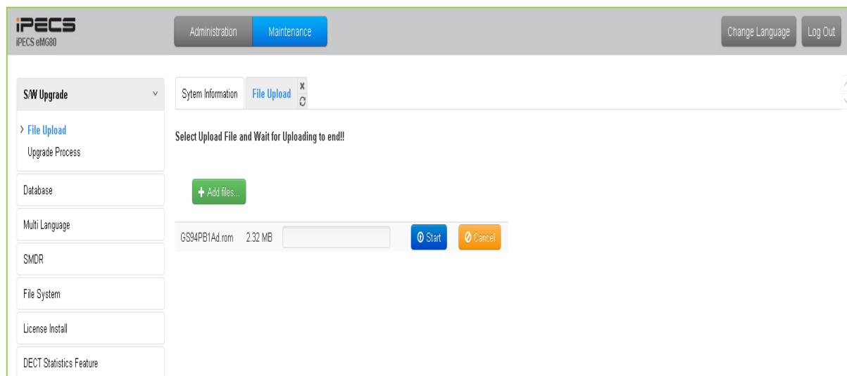
Figure 4.5.1.1-1 File Upload
