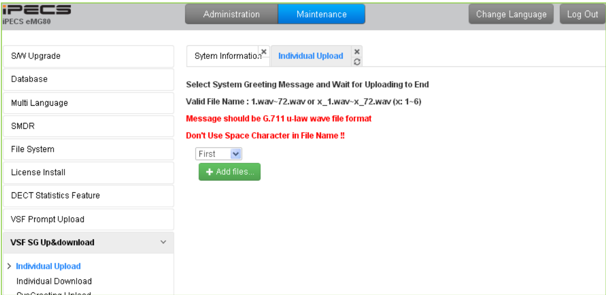
Figure 4.5.9.1-1 Individual Upload
