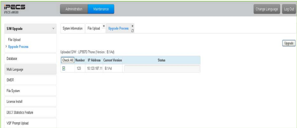
Figure 4.5.1.2-1 Upgrade Process
