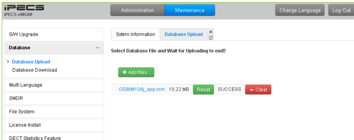
Figure 4.5.2.1-1 Database Upload
