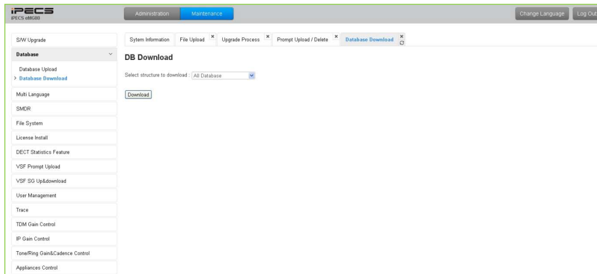
Figure 4.5.2.2-1 Database Download
