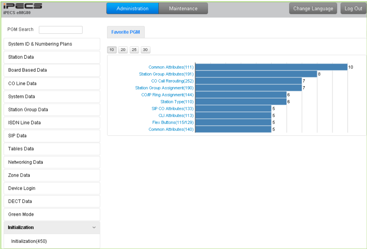
Figure 4.4.15-1 Initialization
