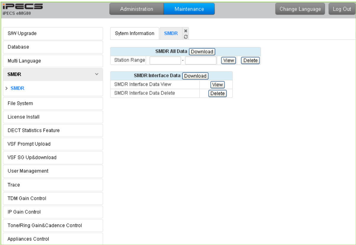
Figure 4.5.4-1 SMDR Access
