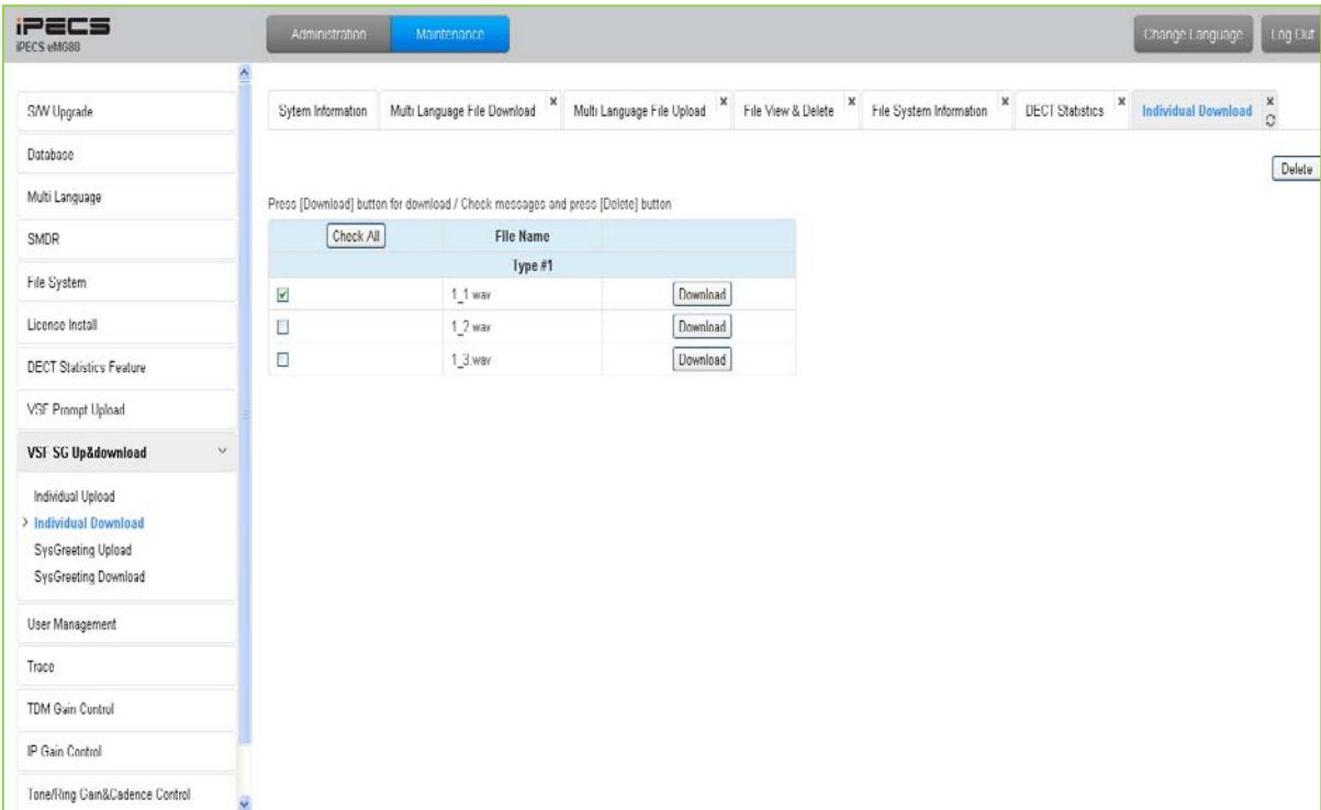
Figure 4.5.9.2-1 Individual Download
