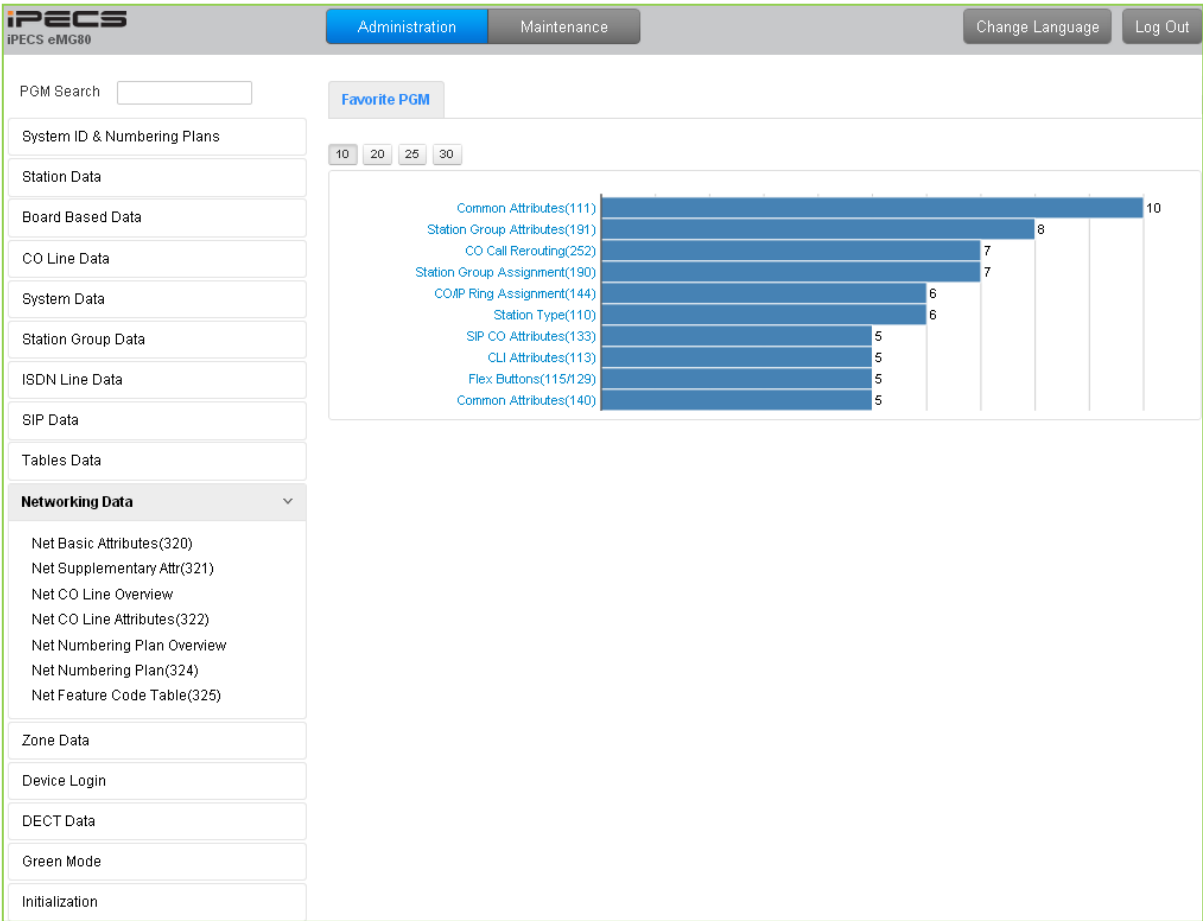
Figure 4.4.10-1 Networking Data
