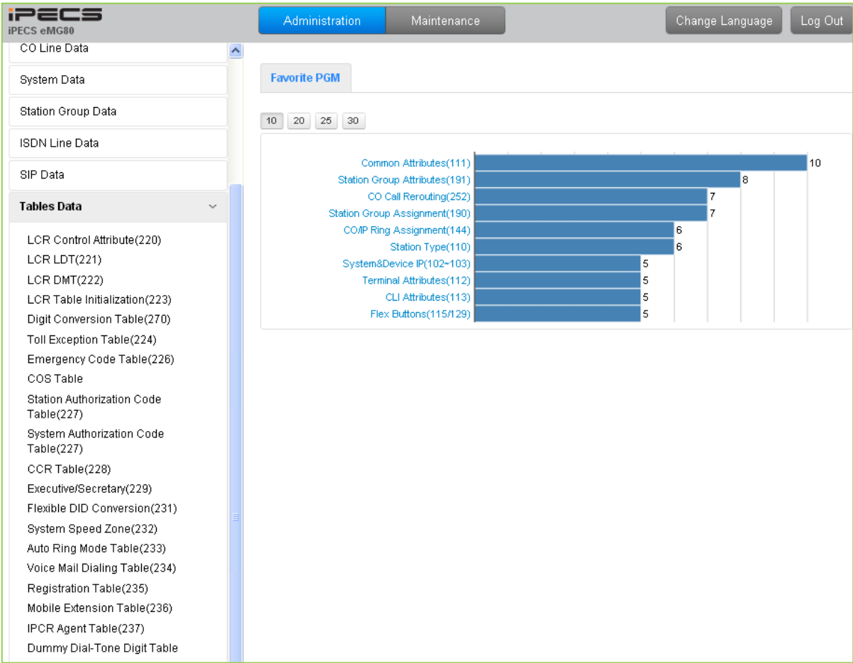
Figure 4.4.9-1 Tables Data
