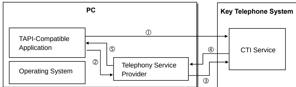
Figure 5.1 Flow of Messages Between the TAPI and TSPI
